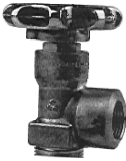
CGA-510 (POL) .880"-14 NGO-L.H. FEMALE
