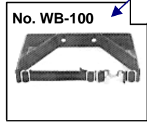
No. WB-100 WALL BRACKET W/ STRAP WIDTH: 10 1/4" DEPTH: 6"
