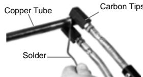
Soldering Joint
