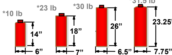
Cylinder Styles (Steel) - (Number = CO2 Fill Weight)
